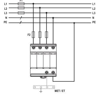
TN-C (Three-phase, 3+0)
