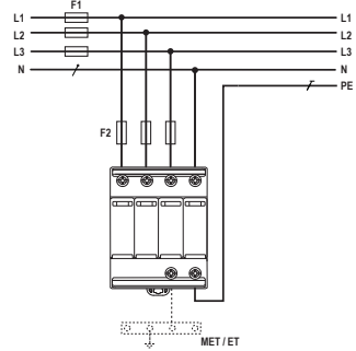
TT (Three-phase, 3+1)
