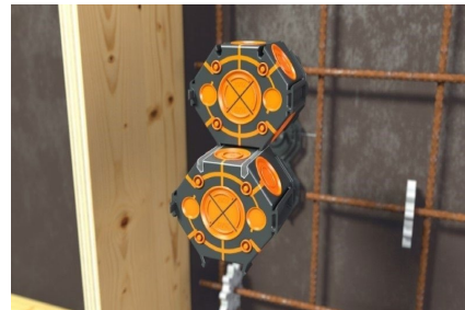
SCS connection technology - fixed connection and simple through-wiring.
