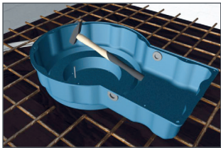
Fix the XL 300 Flex large box with nails to the formwork.
