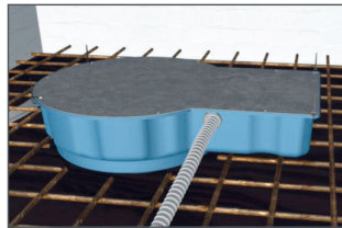
Insert the pipes, close the cover with the cable ties provided.
